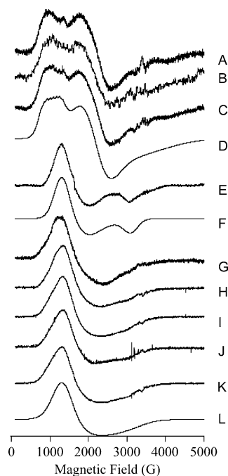
Figure 8. Paramagnetic species that contribute to EPR spectra of ArgE incubated with Co(II). Traces A, B, C, G, H, I, J, and K are difference spectra generated by subtraction of successive experimental spectra from Figure 7, where trace 8A = 7C - 7A, 8B = 7E - 7C, 8C = 7E - 7A, 8E = 7A - 8A, 8G = 7G - 7E, 8H = 7I - 7G, 8I = 7K - 7I, 8J = 7M - 7K, and 8K = 7O - 7M. Trace D is a theoretical spectrum assuming S = 3/2 , M_S = |\pm 1/2\rangle , g_{\parallel} = 2.475 , g_{\perp} = 2.250 , D = 50 \text{ cm}^{-1} (i.e., \gg h\nu ), E/D = 0.25 , A_{\nu}(^{59}\text{Co}) = 9.4 \times 10^{-3} \text{ cm}^{-1} . Trace F is a theoretical spectrum assuming S = 3/2 , M_S = |\pm 1/2\rangle , g_{\parallel} = 2.300 , g_{\perp} = 2.275 , D = 50 \text{ cm}^{-1} (i.e., \gg h\nu ), E/D = 0.08 . Trace L is a theoretical spectrum assuming S = 3/2 , M_S = |\pm 1/2\rangle , g_{\parallel} = 2.200 , g_{\perp} = 2.350 , D = 50 \text{ cm}^{-1} (i.e., \gg h\nu ), E/D = 0.08 .
