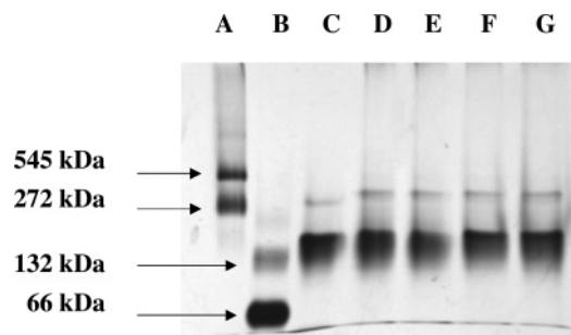
Figure 1. Native PAGE gel of ArgE. The two bands in lane A represent the 272 kDa trimeric and 545 kDa hexameric forms of urease, and the two bands in lane B represent the 66 kDa monomeric and 132 kDa dimeric forms of bovine serum albumin included as molecular weight standards purchased from Sigma. Lanes C–G each contain 8 \mu\text{g} of apo-ArgE that was incubated with varying concentrations of Zn(II). The ArgE in lane C contained no metal. It was dialyzed in 10 mM EDTA and then in 50 mM Chelex 100 treated HEPES, pH 7.5.
