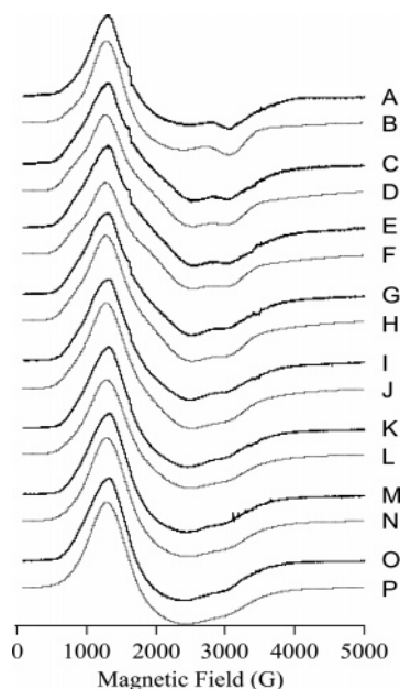
Figure 7. EPR spectra of ArgE were recorded after incubation with 0.21 (A), 0.42 (C), 0.63 (E), 0.84 (G), 1.05 (I), 1.26 (K), 1.47 (M), and 1.68 (O) equiv of Co(II). Traces B, D, F, H, J, L, N, and P are the corresponding computer simulations. The simulations were generated by adding various proportions of the simulated spectra presented in Figure 8, traces D, F, and L. The spin densities accounted for by each component for each of the simulated spectra are presented in Figure 9.
