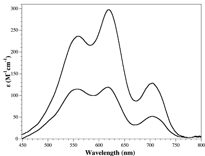
Figure 6. UV-vis absorption spectra of apo-ArgE titrated with 1 (lower) and 2 (upper) equiv Co(II) to form [Co•(ArgE)] and [CoCo(ArgE)], respectively. Spectra were recorded with 1 mM enzyme in HEPES buffer pH 7.5.
