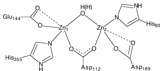
Figure 10. Proposed active site of the ArgE from E. coli based on sequence alignments with AAP and CPG 2 .
