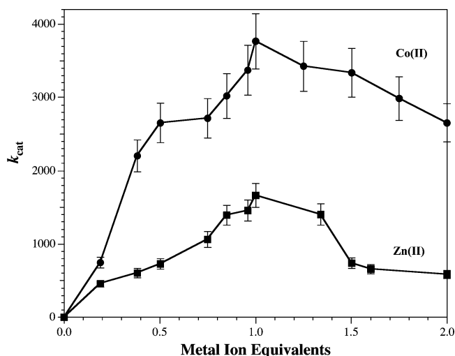
Figure 2. k_{\text{cat}} of a 10\text{ }\mu\text{M} apo-ArgE titrated with 0.2–2.0 equiv of Zn(II) or Co(II).
